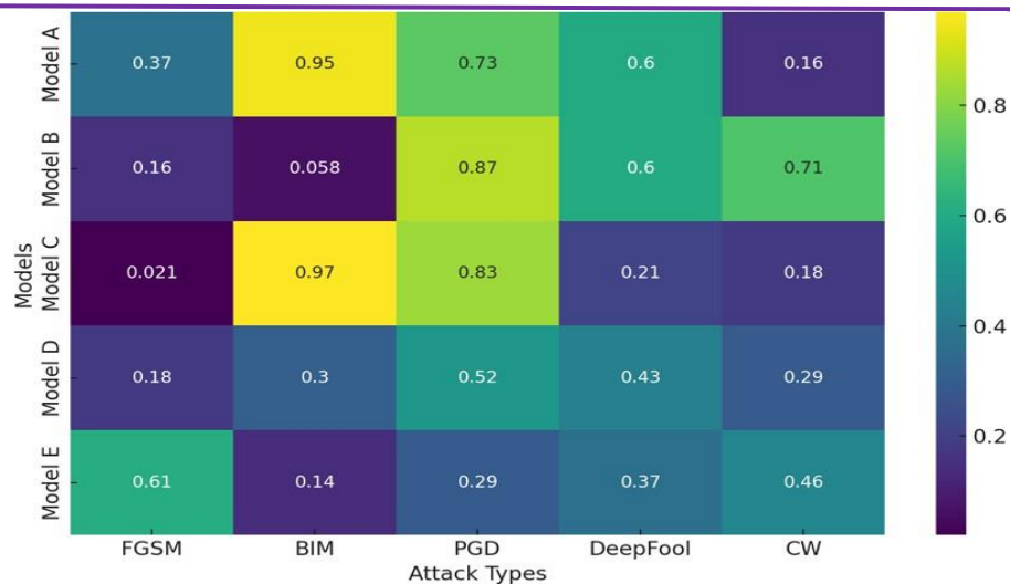
Figure 3. Robustness against adversarial attacks
