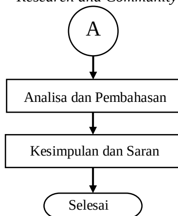
Gambar 1. Flowchart Penelitian
