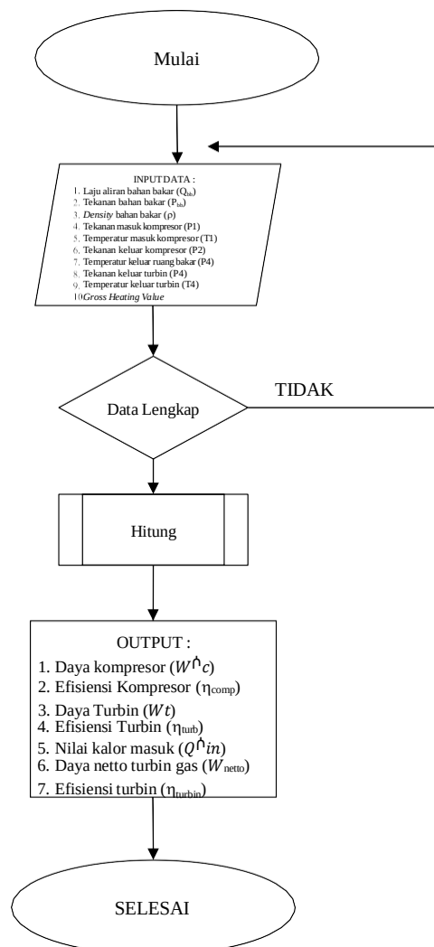
Gambar 1. Flowchart Program
