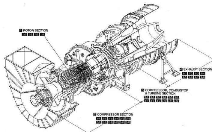
Gambar 2. Gas Turbin M701D
