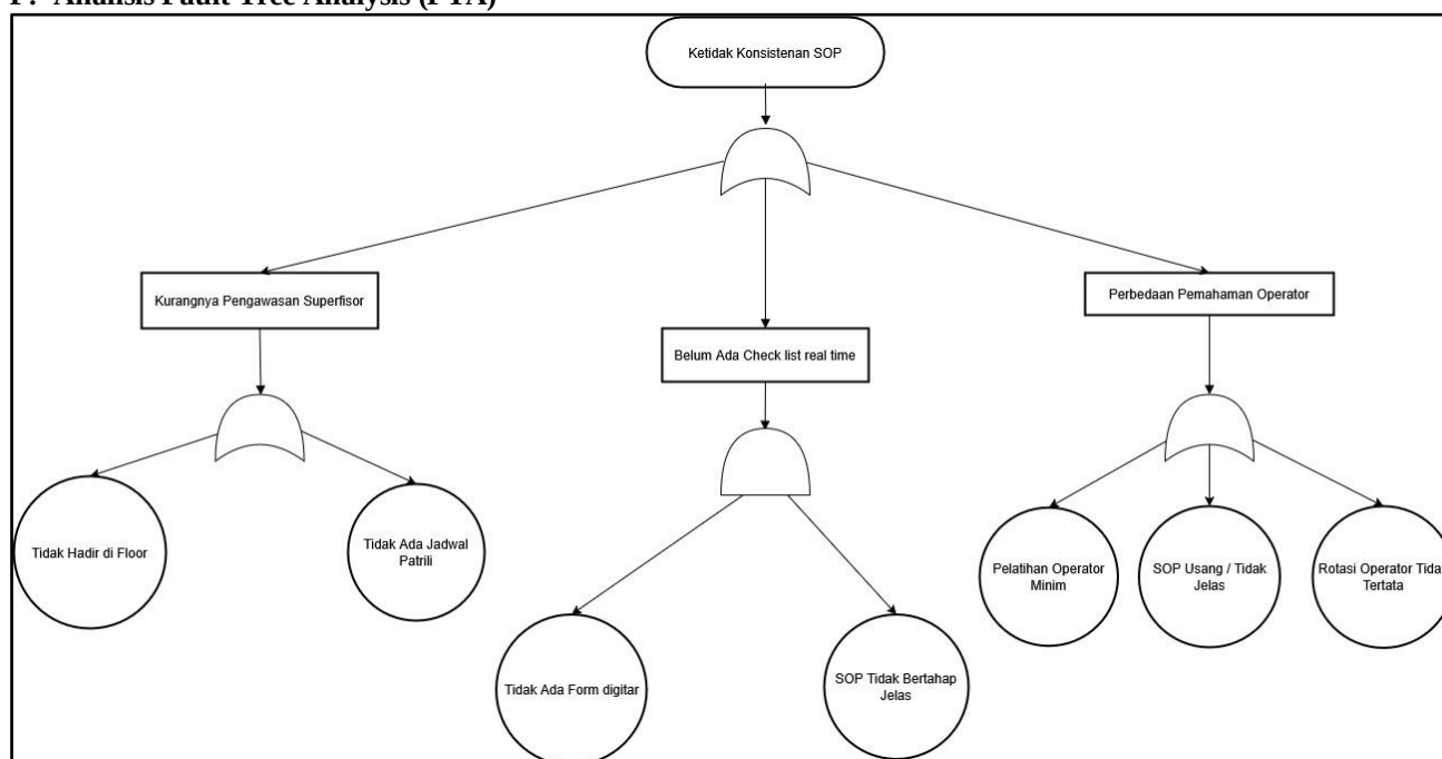
Gambar 3 Fault Tree Analisis Diagram
