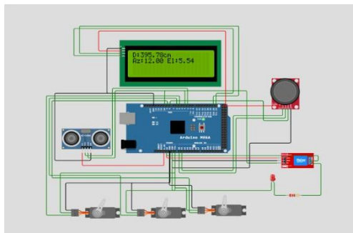
rangkaian firing control mencari target
