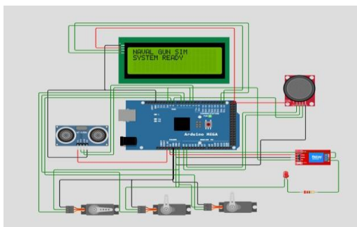
rangkaian firing control saat on
