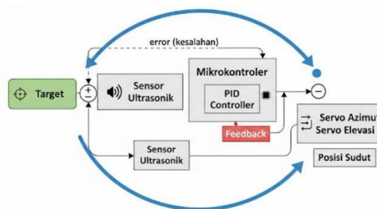
1.5.1 diagram Blok (closed-loop control).
