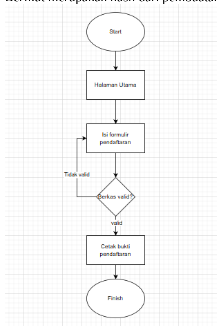
Gambar 6. User Flow
