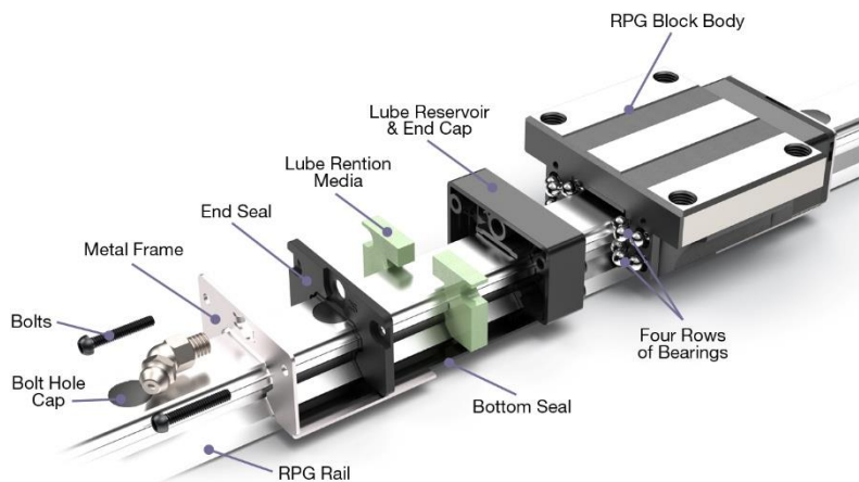
Gambar 2. Linear bearing
