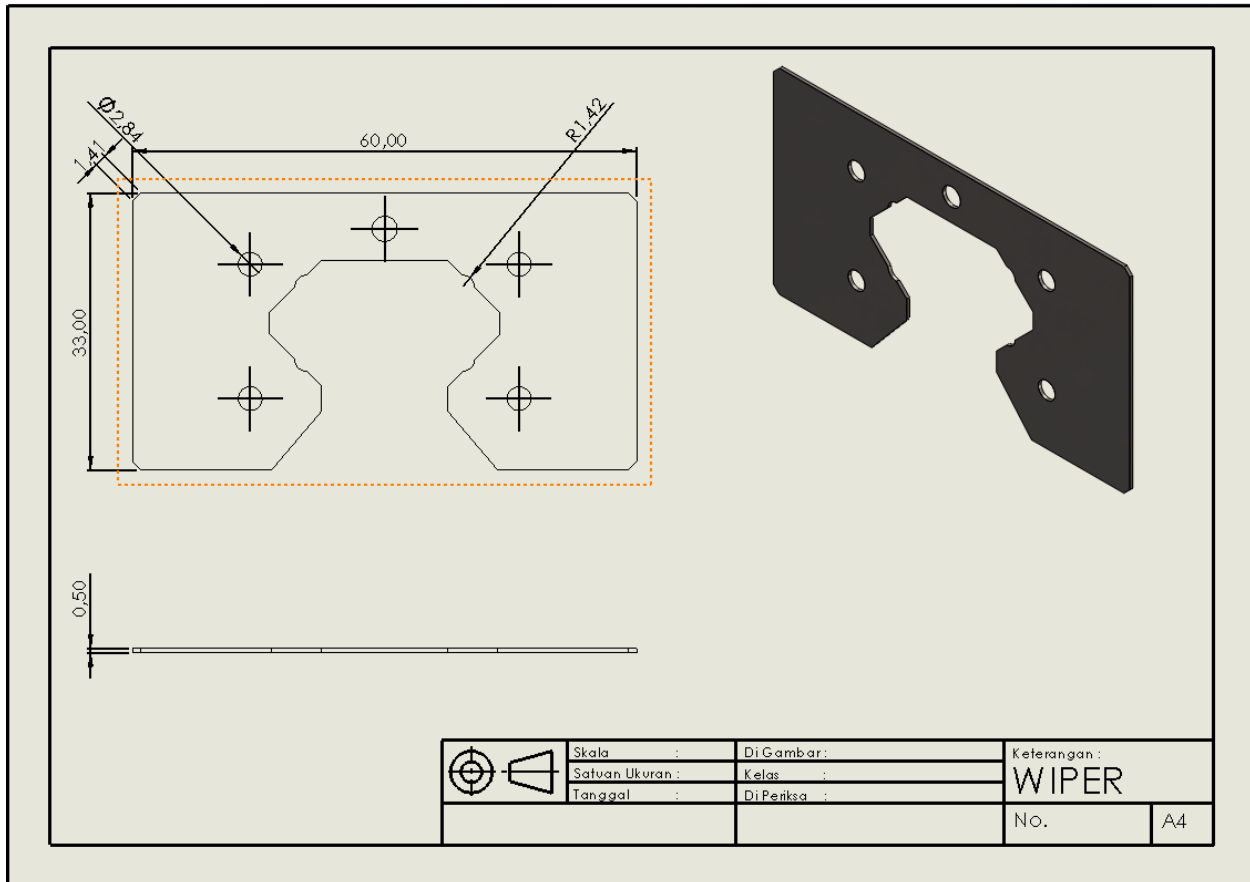
Gambar 5. Design Wiper
