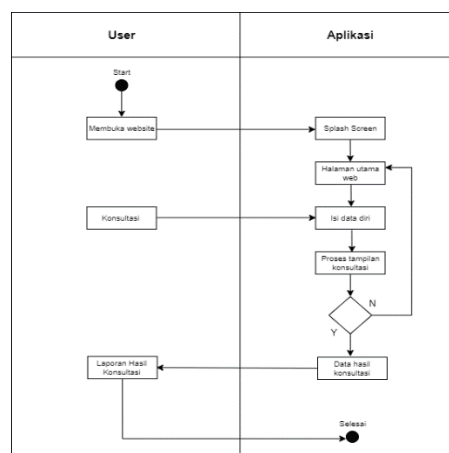
Gambar 4. Activity Diagram
