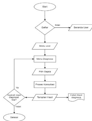
Gambar 2. Flowchart
