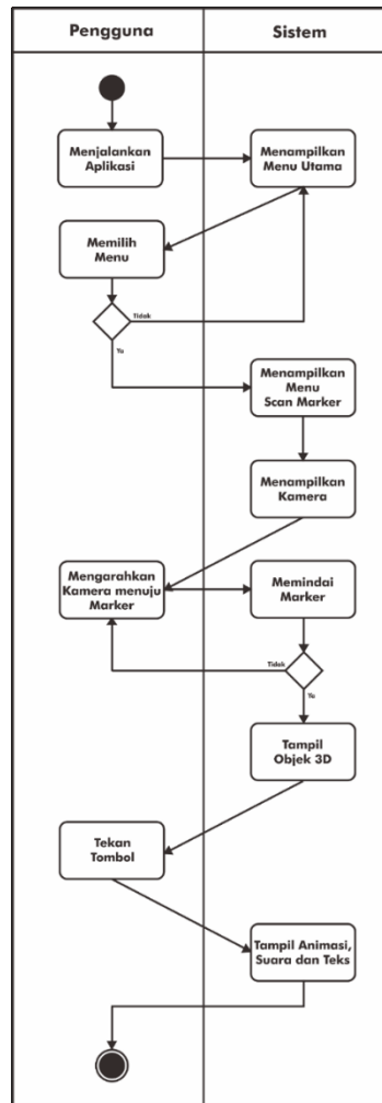
Gambar 5. Activity Diagram
